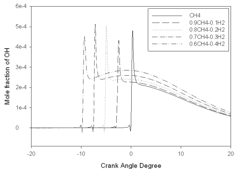
Fig.10. Effect of addition of \text{H}_2 to \text{CH}_4 on radical OH
